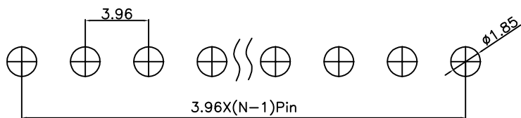
PCB LAYOUT
