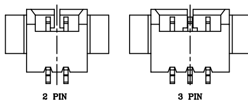
LOCK CONFIGURATION
