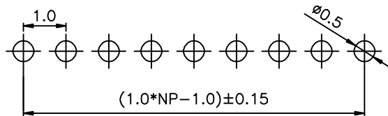
PCB LAYOUT
